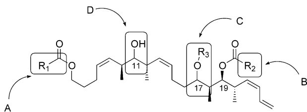
Figure 2. Simplified analogues of discodermolide: domains of variation.
