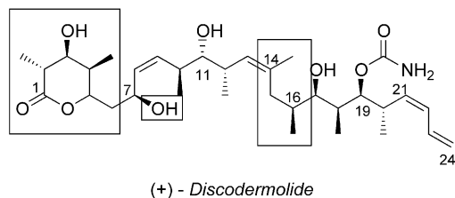
Figure 1. Discodermolide with areas targeted for simplification in boxes.
